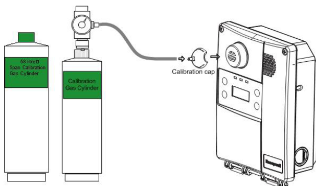
Figure 9. Calibration Installation
