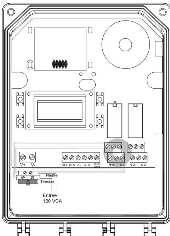
Illustration 5. 120 VCA Connection
